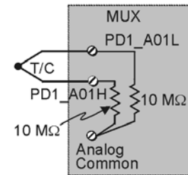
Example of Floating Differential Circuit
