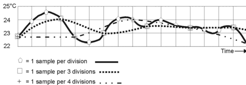
Examples of Under Sampling
