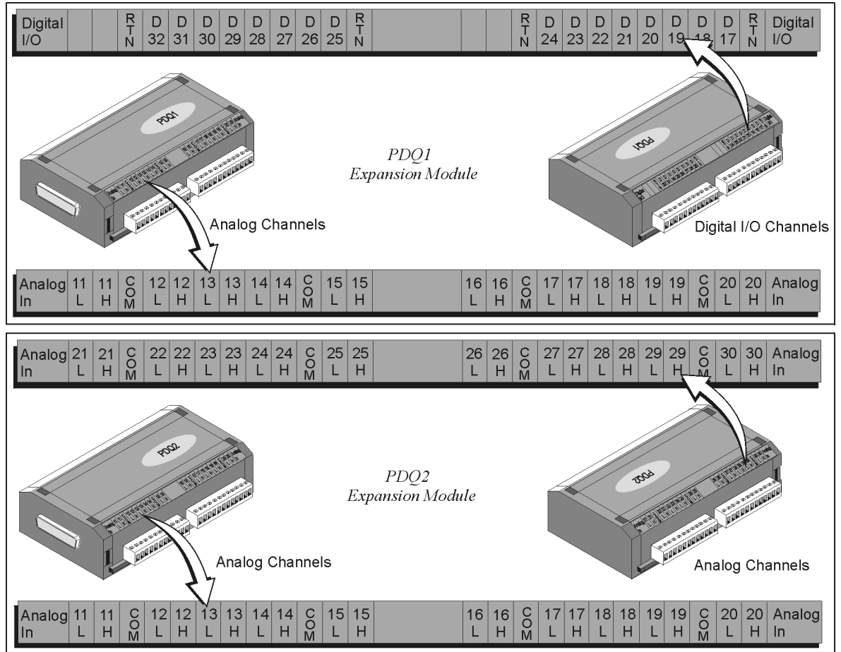
Channel Connection Layouts
